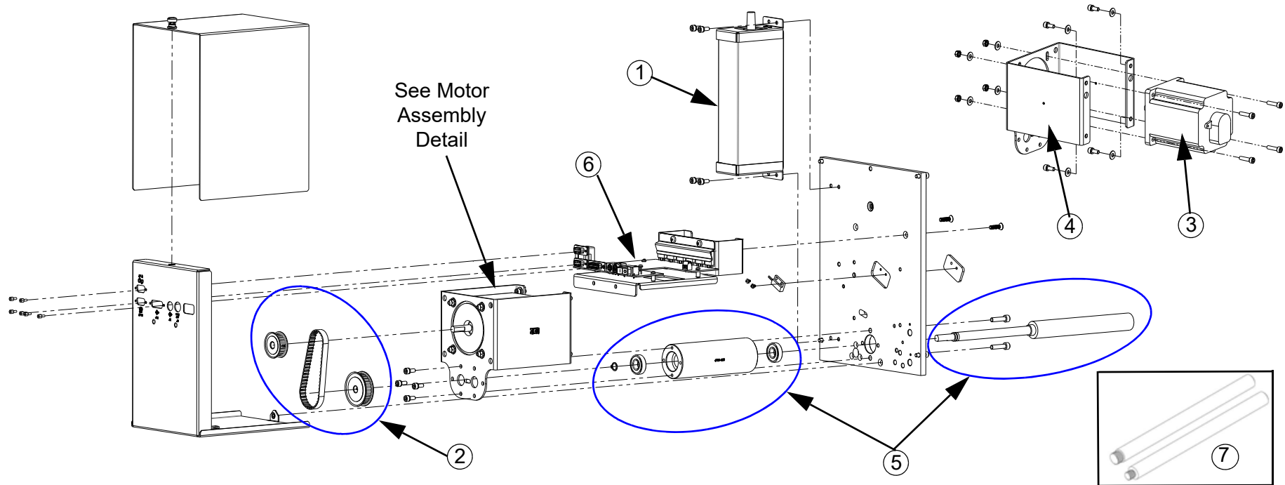
Motor Assembly Detail
